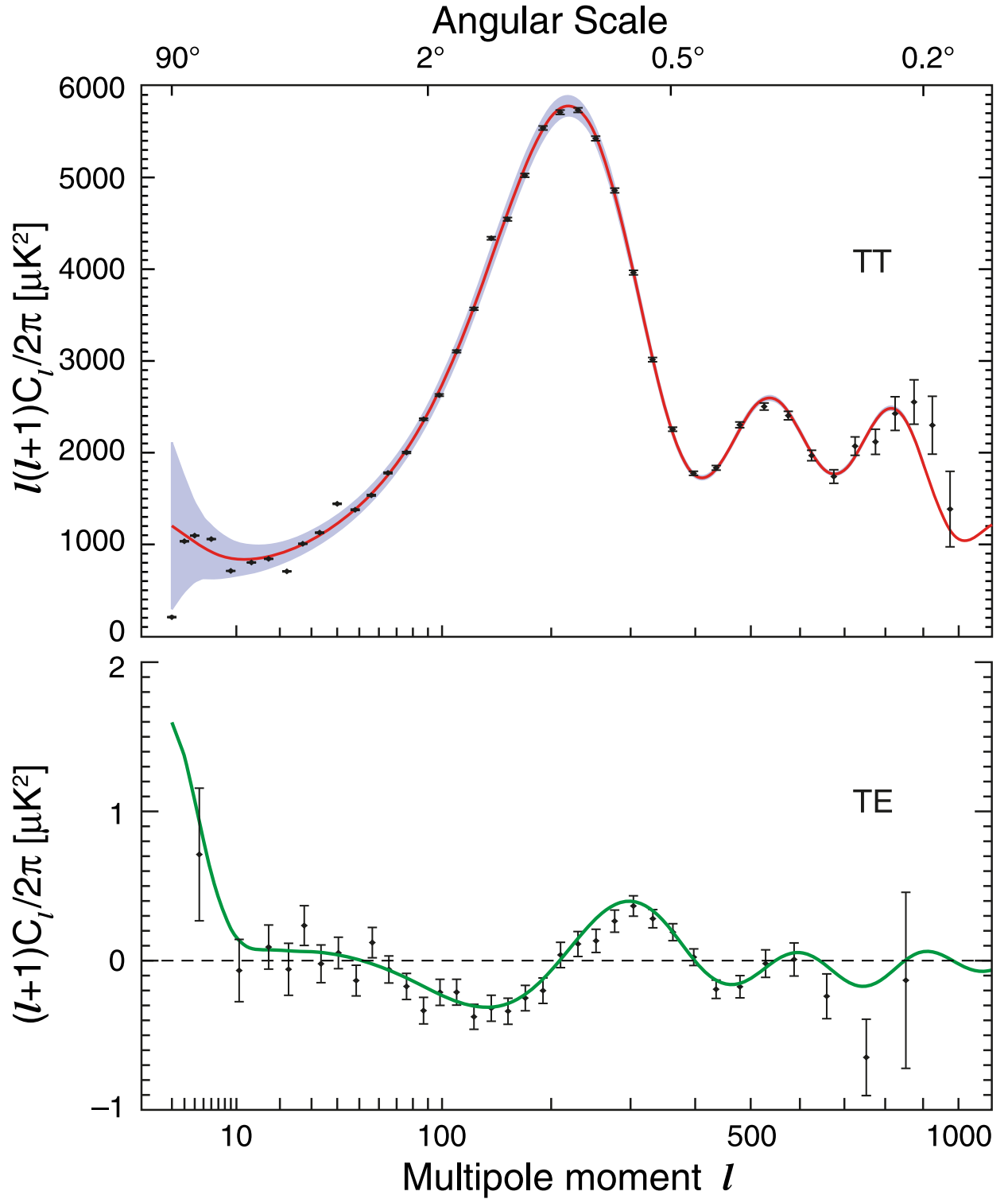
Fig. 13.— The temperature (TT) and temperature-polarization correlation (TE) power spectra based on the 5 year WMAP data. The addition of 2 years of data provide more sensitive measurements of the third peak in TT and the high- l TE spectrum, especially the second trough.
