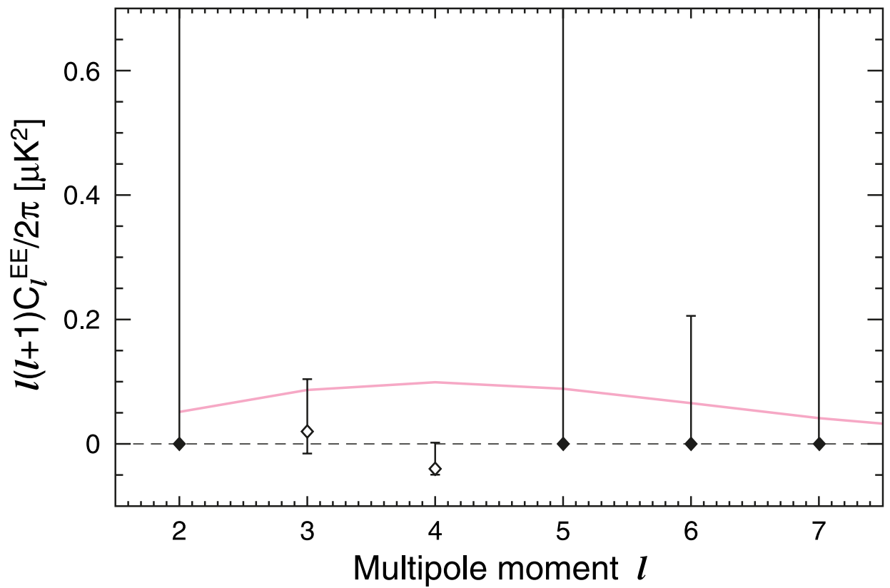
Fig. 10.— The EE power spectrum computed from the null sky maps, \frac{1}{2}S_{K_a} - \frac{1}{2}S_{Q_V} , where S = Q, U are the polarization Stokes parameters, and S_{Q_V} is the optimal combination of the Q and V band data. The pink curve is the best-fit theoretical spectrum from Dunkley et al. (2008). The spectrum derived from the null maps is consistent with zero.
