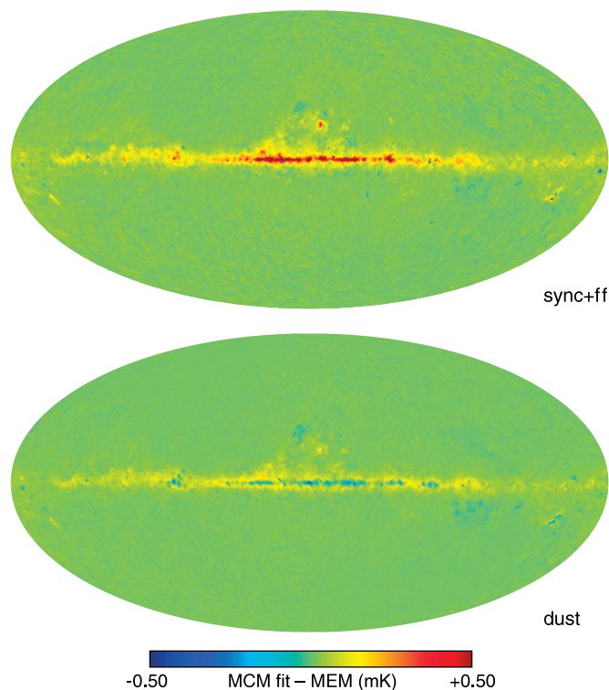
Figure 11. Difference between the MCMC fit and MEM maps. The top panel is the difference (at the K band) in synchrotron plus free–free emission. Differences between these two components separately are larger due to the degeneracy direction. The bottom panel is the difference (at the W band) in the dust maps. The differences are roughly 1% of total emission at the K band and a few percent at the W band.
