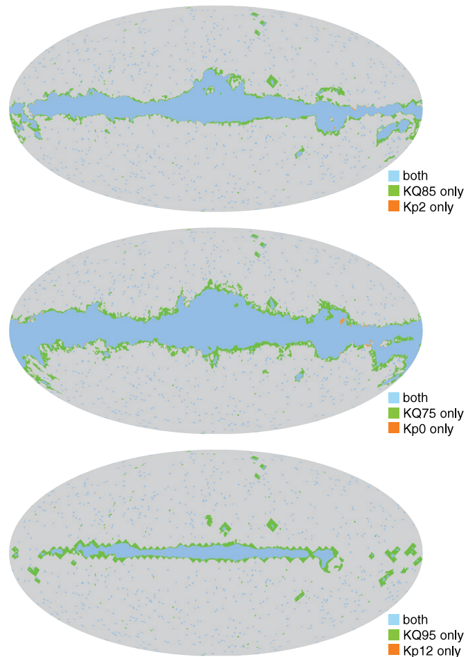
Figure 1. Comparison maps of the 5 year masks vs. the 3 year masks. The new masks cover slightly more of the Galactic plane and cover more regions with low synchrotron but high free–free emission. The diamond-shaped features arise because the new processing mask has been defined to correspond to low-resolution ( N_{\text{side}} = 16 ) pixels, so that the same processing mask can be used at all resolutions. Top: comparison of KQ85 with the 3 year Kp2 mask. Middle: comparison of KQ75 with the 3 year Kp0 mask. Bottom: comparison of KQ95 with the 3 year Kp12 mask.
