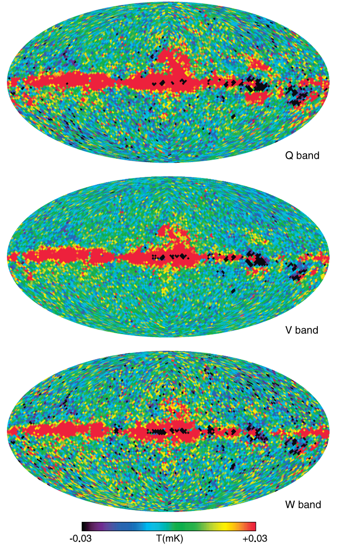
Figure 4. 5 year temperature maps with foregrounds reduced via template cleaning. All maps have had the 5 year ILC estimate for the CMB subtracted, and have been degraded to N_{\text{side}} = 32 . Frequency bands shown are Q, V, and W. Compare to Figure 10 of Hinshaw et al. (2007). Outside the Galactic mask, the template cleaning reduces foregrounds to \sim 15 \mu\text{K} or less.
