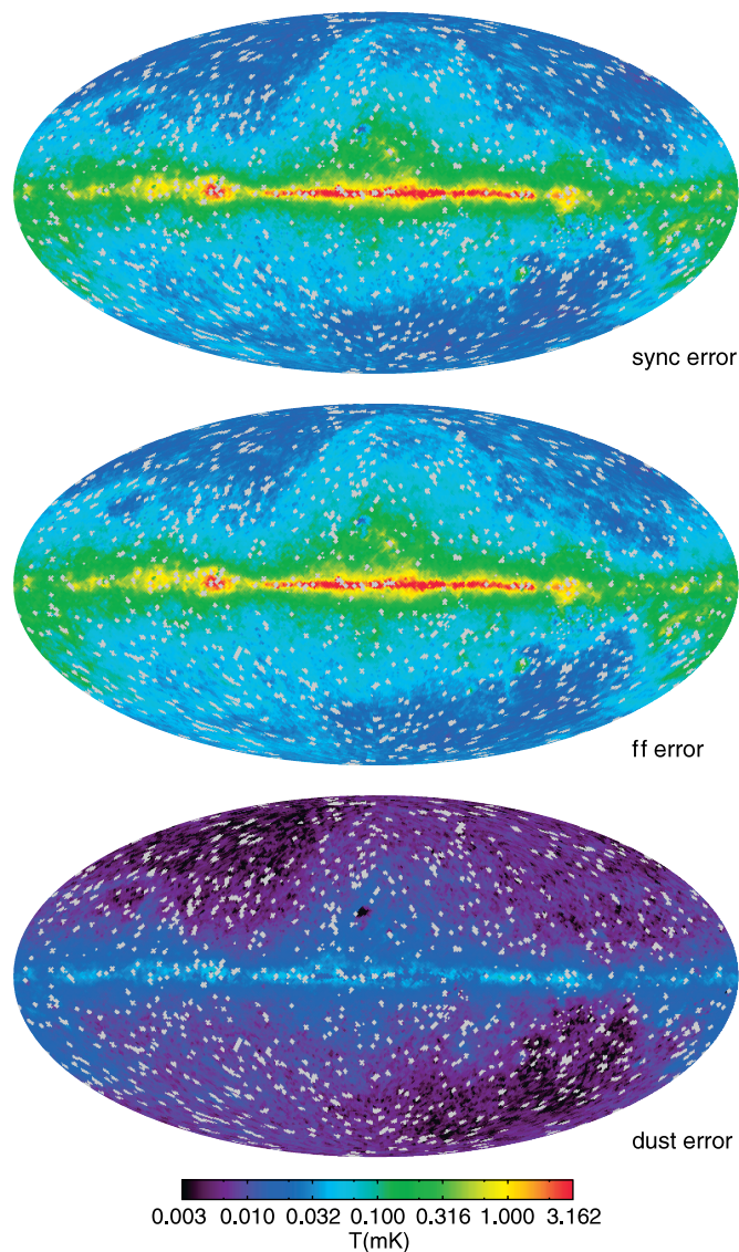
Figure 12. Error maps for foreground components as determined from the marginalized variance given by the MCMC fitting process. Error maps for synchrotron and free–free emission are similar due to the parameter degeneracy between them. Synchrotron and free–free temperatures are as measured at the K band; dust is measured at the W band. Gray pixels are those masked due to point sources or flagged as problematic. Top: synchrotron, middle: free–free, bottom: dust.
