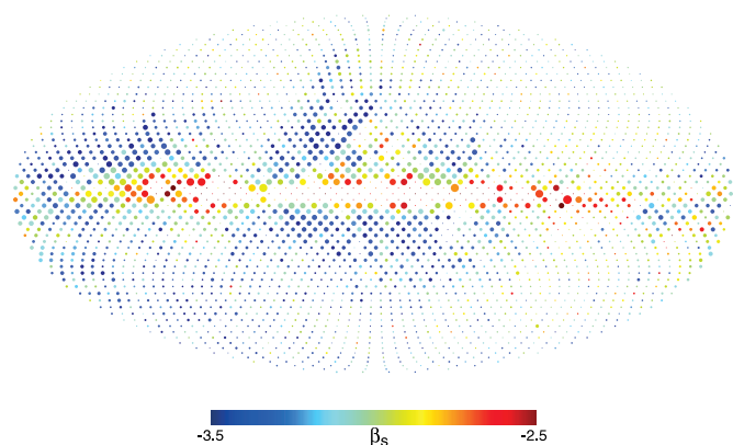
Figure 13. Map of the synchrotron spectral index for the “base” fit, binned to N_{\text{side}} = 16 . Color shows the value of the spectral index and the circle area indicates the weight \sigma_{\beta}^{-2} given by the fit. Pixels with \chi^2 > 2 were explicitly deweighted.
