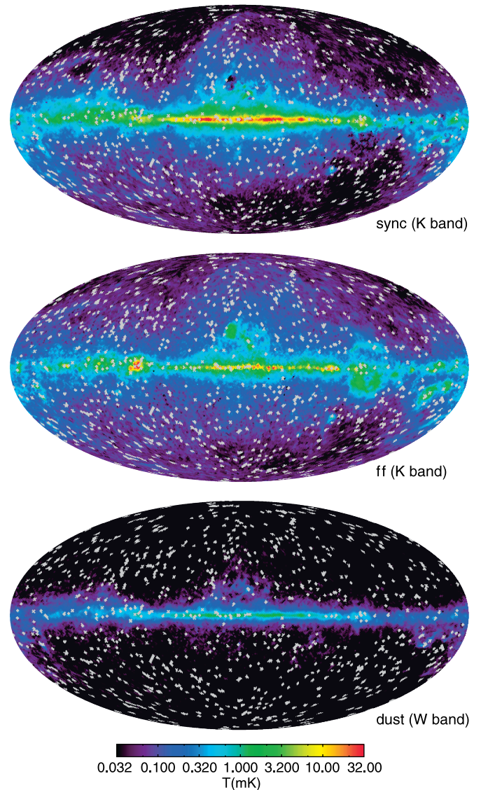
Figure 9. Temperature maps for foreground components as determined by the MCMC fitting process for the ‘‘base’’ model. Maps from other models are qualitatively similar. Synchrotron and free–free temperatures are as measured at the K band; dust is measured at the W band. Gray pixels are those masked due to point sources or flagged as problematic. Top: synchrotron, middle: free–free, bottom: dust.
