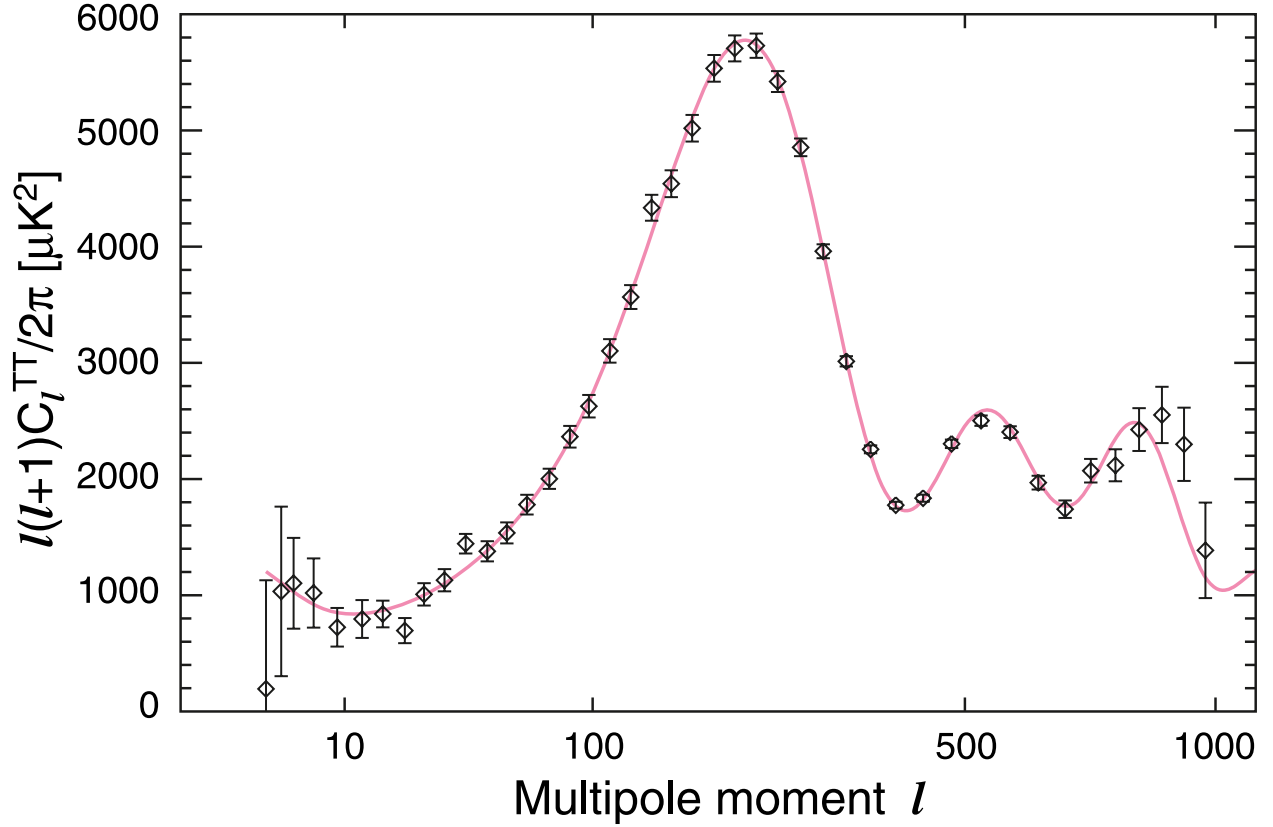
Fig. 1.— The WMAP 5-year temperature (TT) power spectrum. The red curve is the best-fit theory spectrum from the \Lambda CDM/ WMAP chain (Dunkley et al. 2008, Table 2) based on WMAP alone, with parameters (\Omega_b h^2, \Omega_m h^2, \Delta_{\mathcal{R}}^2, n_s, \tau, H_0) = (0.0227, 0.131, 2.41, 0.961, 0.089, 72.4) . The uncertainties include both cosmic variance, which dominates below \ell = 540 , and instrumental noise which dominates at higher multipoles. The uncertainties increase at large \ell due to WMAP 's finite resolution. The improved resolution of the third peak near \ell = 800 in combination with the simultaneous measurement of the rest of the spectrum leads to the improved results reported in this release.
