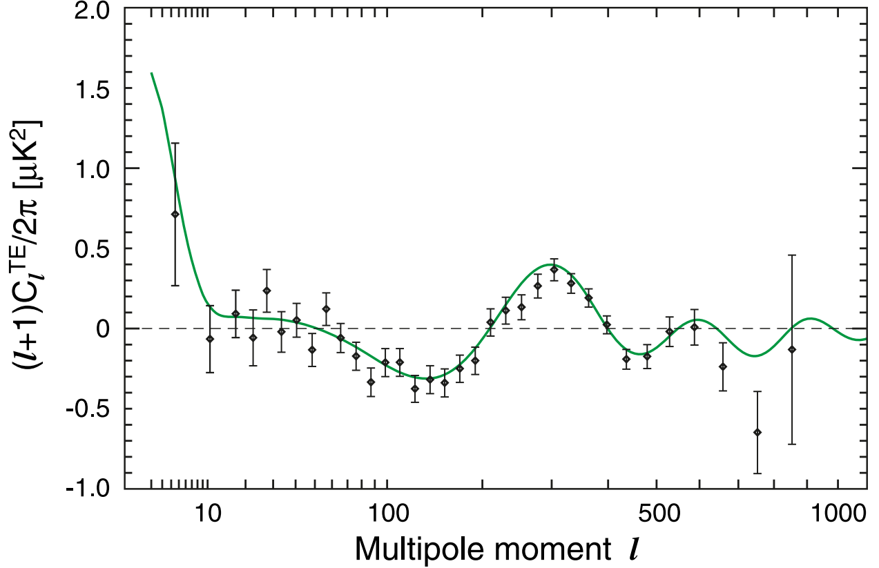
Fig. 5.— The WMAP 5-year TE power spectrum. The green curve is the best-fit theory spectrum from the \Lambda CDM/ WMAP Markov chain (Dunkley et al. 2008). For the TE component of the fit, \chi^2 = 415 , and there are 427 multipoles and 6 parameters; thus the number of degrees of freedom is \nu = 421 , leading to \chi^2/\nu = 0.99 . The particle horizon size at decoupling corresponds to l \approx 100 . The clear anticorrelation between the primordial plasma density (corresponding approximately to T) and velocity (corresponding approximately to E) in causally disconnected regions of the sky indicates that the primordial perturbations must have been on a superhorizon scale. Note that the vertical axis is (\ell + 1)C_\ell/(2\pi) , and not \ell(\ell + 1)C_\ell/(2\pi) .
