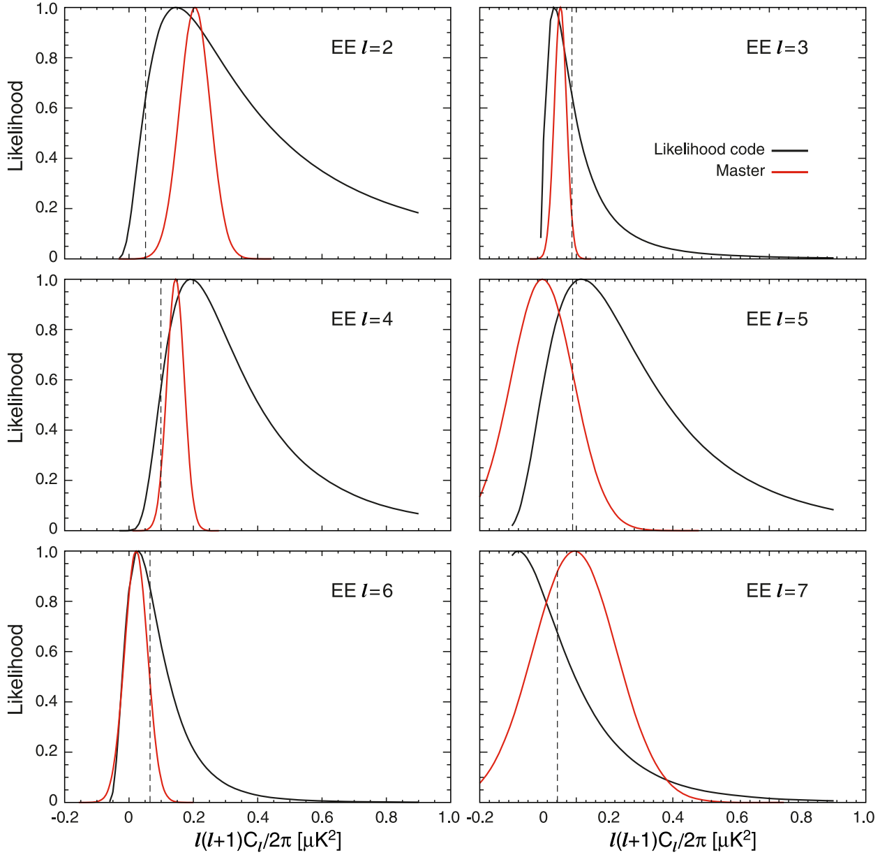
Fig. 7.— Conditional likelihoods for the \ell = 2 - 7 EE multipole moments (black curves), computed using the WMAP likelihood code by varying the multipole in question, with all other multipoles fixed to their fiducial values. For example, in the \ell = 4 panel, the black curve is f(x) \propto L(d) \dots, C_3^{EE}, C_4^{EE} = x, C_5^{EE}, \dots . For comparison, naive pseudo- C_\ell estimates are also shown with Gaussian errors (red curves). The pseudo- C_\ell errors are noise only, while the conditional distributions include cosmic variance.
