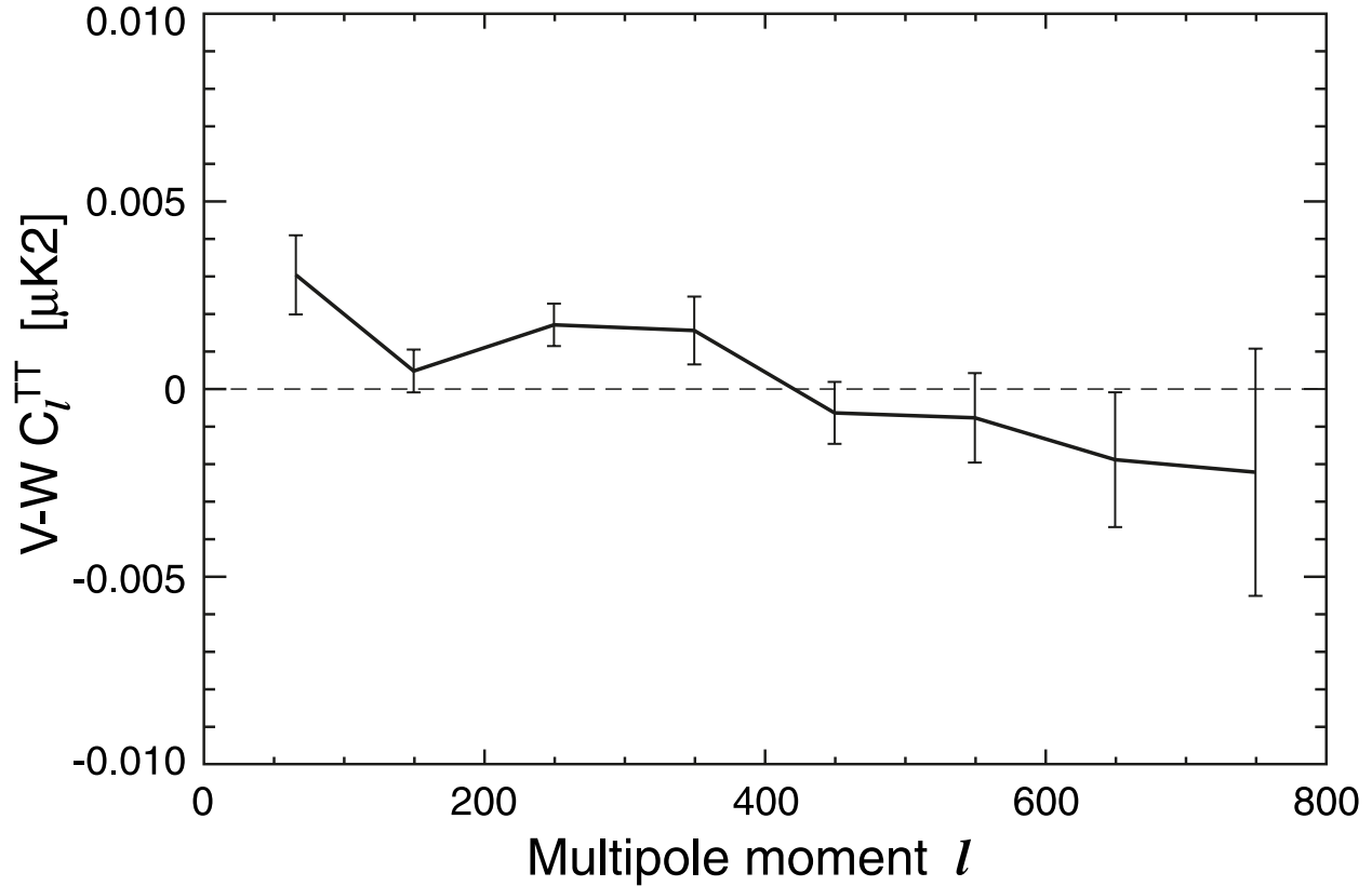
Fig. 4.— The TT V - W null spectrum. After correcting for unresolved point source emission, the individual power spectra are subtracted in power spectrum space. The result is consistent with zero and thus there is no evidence of point source contamination. In these units, point source contamination would be evident as a horizontal offset from zero. At l = 500 , the TT power spectrum is C_l^{TT} \approx 0.06 ; thus the contamination is limited to roughly 3% in power.
