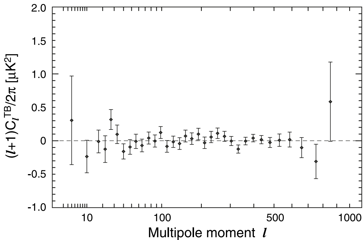
Fig. 6.— The WMAP 5-year TB power spectrum, showing no evidence of cosmological signal. The null reduced \chi^2 for \ell = 24 - 450 is 0.97. Note that the vertical axis is (\ell + 1)C_\ell/(2\pi) , and not \ell(\ell + 1)C_\ell/(2\pi) .
