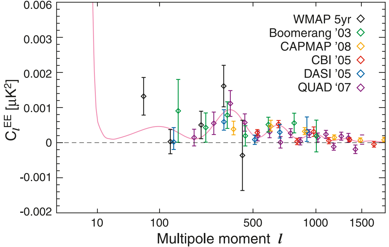
Fig. 10.— WMAP 5-year EE power spectrum, compared with results from the Boomerang (Montroy et al. 2006, green), CAPMAP (Bischoff et al. 2008, orange), CBI (Sievers et al. 2007, red), DASI (Leitch et al. 2005, blue), and QUAD (P. Ade et al. 2007, purple) experiments. The pink curve is the best-fit theory spectrum from the \Lambda CDM/ WMAP Markov chain (Dunkley et al. 2008). Note that the y -axis is C_l^{EE} , not \ell(\ell + 1)C_\ell^{EE}/(2\pi) .
