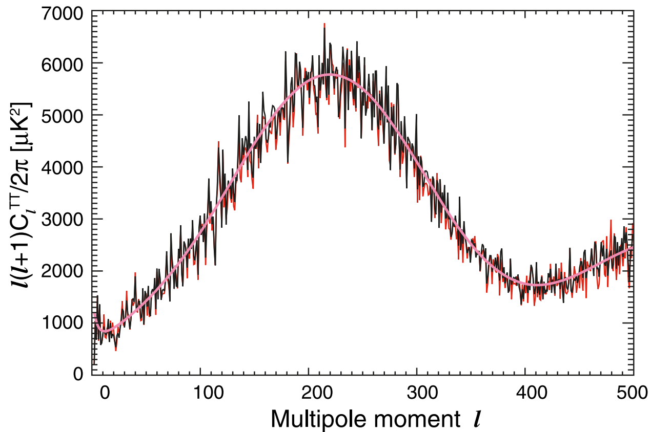
Fig. 12.— The unbinned WMAP 5-year temperature (TT) power spectrum (black), compared with the WMAP 3-year result (red). The slight upward shift of the 5-year spectrum relative to the 3-year spectrum is due to the change in the beam transfer function. The pink curve is the best-fit \Lambda CDM model to the WMAP 5 data.
