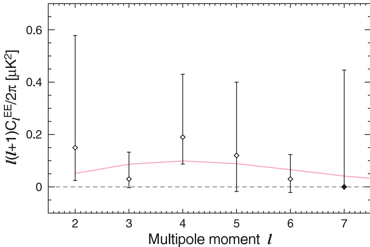
Fig. 9.— WMAP 5-year EE power spectrum at low- l . The error bars are the 68% CL of the conditional likelihood of each multipole, with the other multipoles fixed at their fiducial theory values; the diamonds mark the peak of the conditional likelihood distribution. The error bars include noise and cosmic variance; the point at l = 7 is the 95% CL upper limit. The pink curve is the fiducial best-fit \Lambda CDM model (Dunkley et al. 2008).
