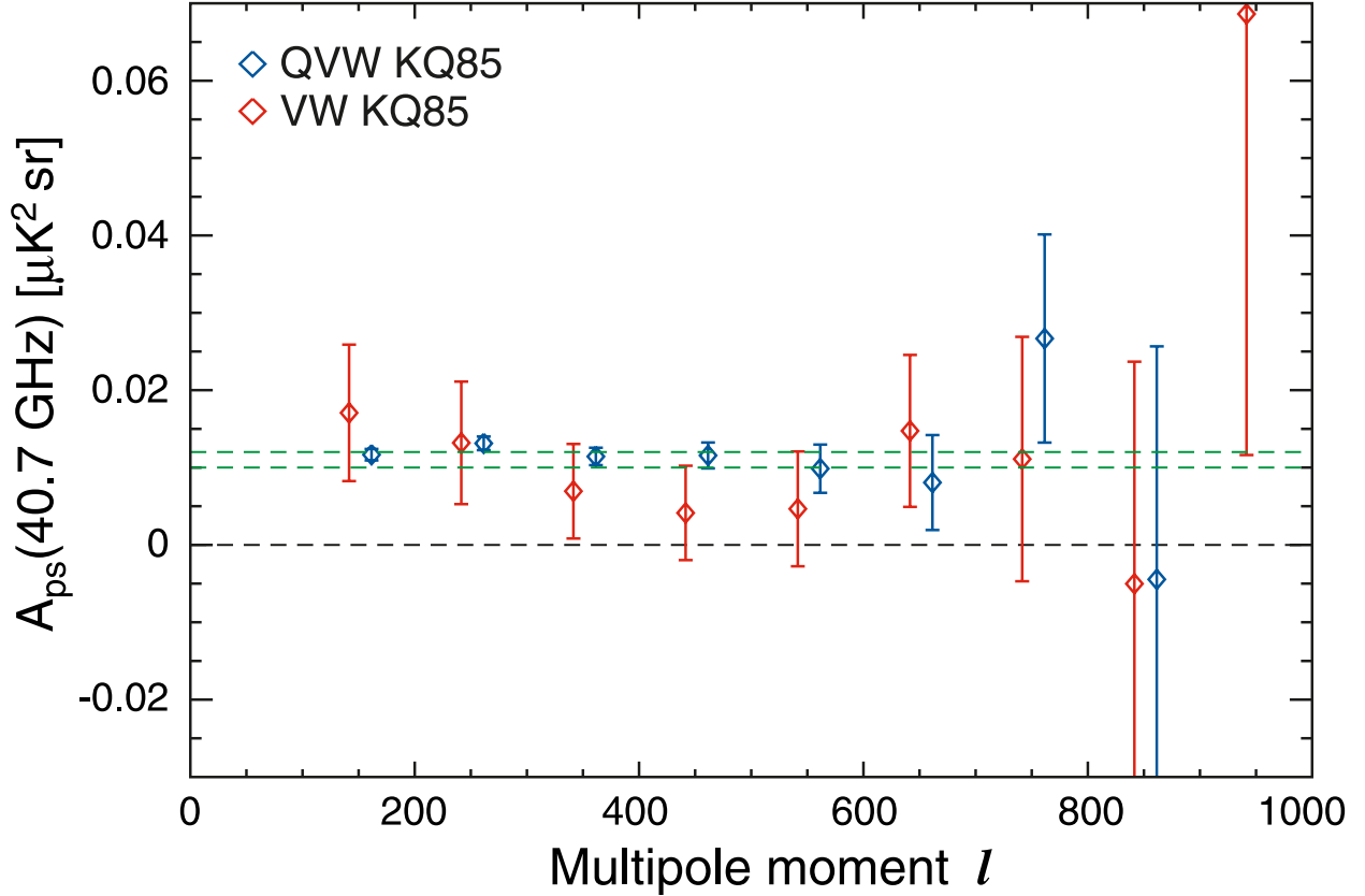
Fig. 3.— The unresolved point source contamination A_{ps} , measured in bins of \Delta\ell = 100 evaluated at 40.7 GHz (Q-band). For a source population whose fluxes are independent of frequency A_{ps} scales roughly as \sim \nu^{-2} in the WMAP data. The red data points are from the analysis of V and W bands alone and the blue points are from the analysis of Q, V, and W bands. The horizontal dashed green lines, at 0.010 and 0.012, show the 1\sigma bounds for our adopted value of A_{ps} . Note that the QVW amplitude is independent of \ell .
