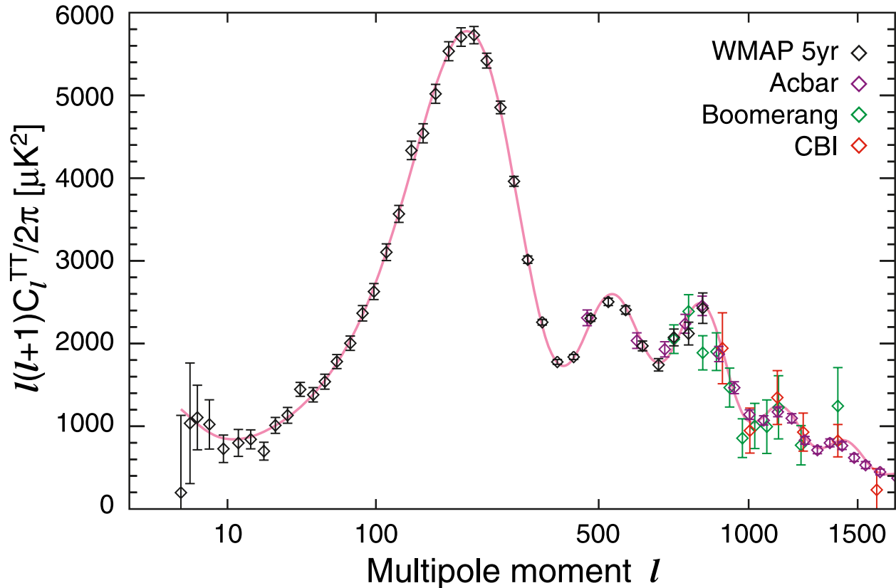
Fig. 2.— The WMAP 5-year TT power spectrum along with recent results from the ACBAR (Reichardt et al. 2008, purple), Boomerang (Jones et al. 2006, green), and CBI (Readhead et al. 2004, red) experiments. The other experiments calibrate with WMAP or WMAP ’s measurement of Jupiter (CBI). The red curve is the best-fit \Lambda CDM model to the WMAP data, which agrees well with all data sets when extrapolated to higher- l .
