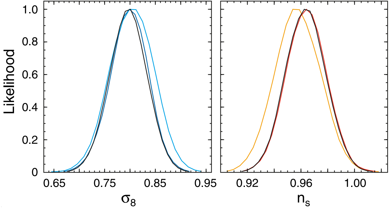
Fig. 11.— Left: One-dimensional marginalized likelihood distributions of \sigma_8 for various treatments of the source uncertainty in the likelihood code: the standard likelihood function [black], the alternative treatment of the source uncertainty described in equation (A5) [blue], the alternative treatment, but with the unresolved point source error increased by \times 5 [cyan]. The agreement between black and blue curves shows that the standard treatment is producing the correct answer. Right: 1D marginalized likelihood distributions of n_s for various treatments of the beam uncertainties: the standard likelihood function [black], the alternative treatment of the beam uncertainty described in equation (A5) [red], the alternative treatment, but with the beam error increased by a factor of 20 [orange]. The agreement between the black and red curves shows that the standard treatment is producing the correct answer.
