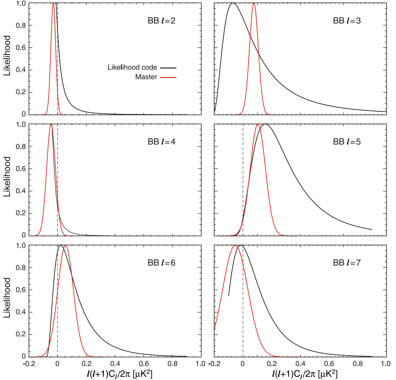
Fig. 8.— Conditional likelihoods for the \ell = 2 - 7 BB multipole moments (black curves), computed using the WMAP likelihood code by varying the multipole in question, with all other multipoles fixed to their fiducial values. For comparison, naïve pseudo- C_\ell estimates are also shown with Gaussian errors (red curves). The pseudo- C_\ell errors are noise only, while the conditional distributions include cosmic variance. Note the large difference between the likelihood code and the pseudo- C_\ell value for \ell = 3 ; this mode is sensitive to the time-ordered data baseline and is extremely poorly measured by WMAP , illustrating the complicated noise structure of the polarization data on large scales.
